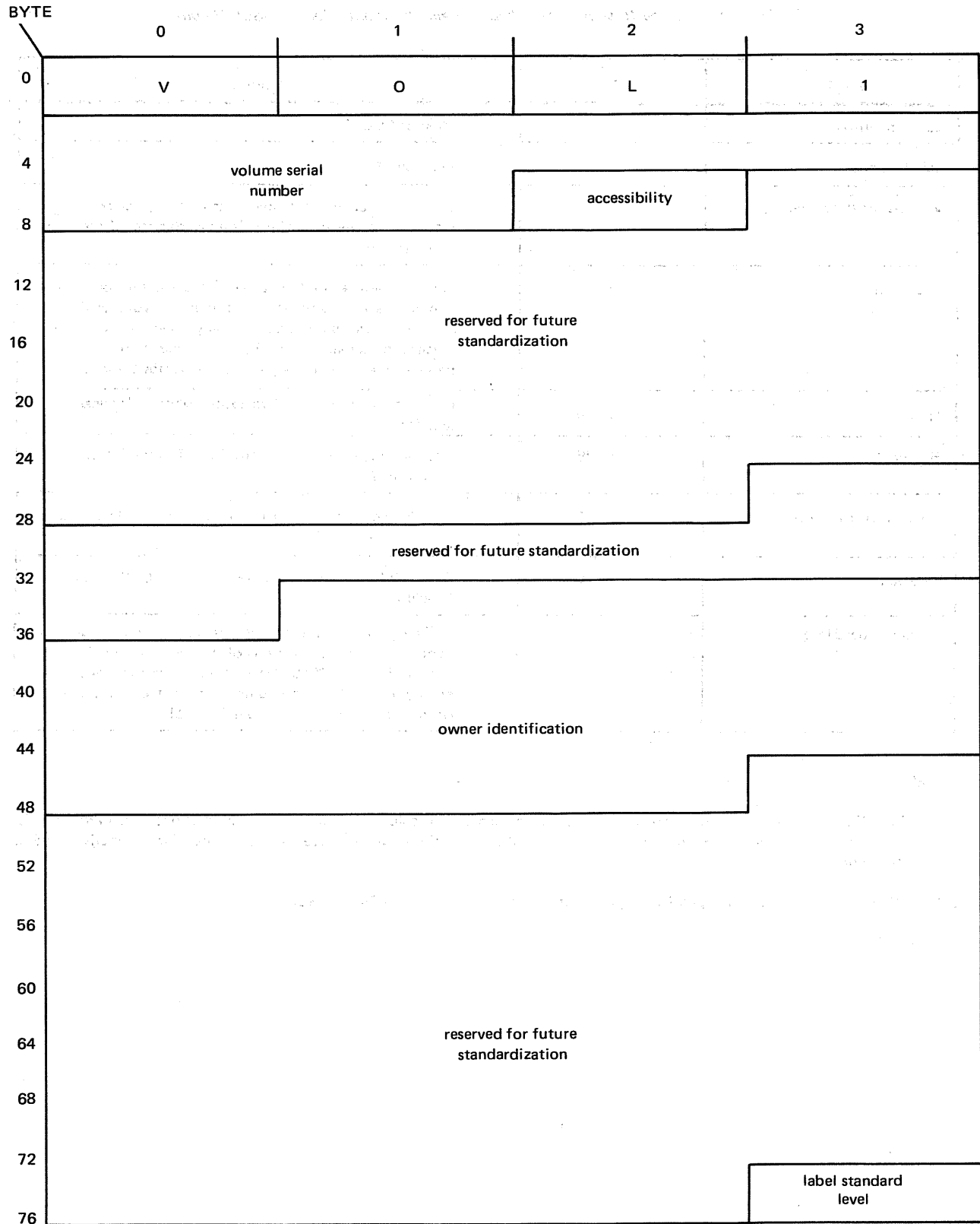
Figure E-7. Volume Header Label (VOL1) for an ASCII Magnetic Tape Volume
