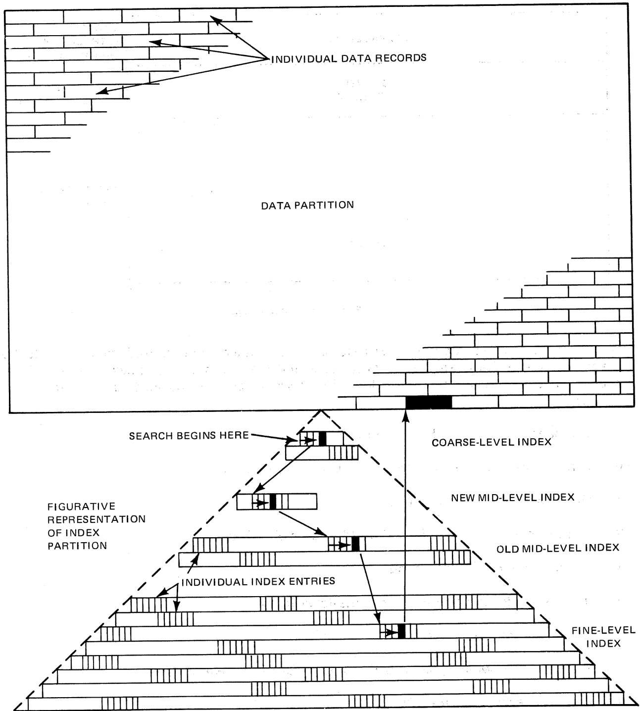
Figure 12-6. Typical Search of 4-Level IRAM Index
