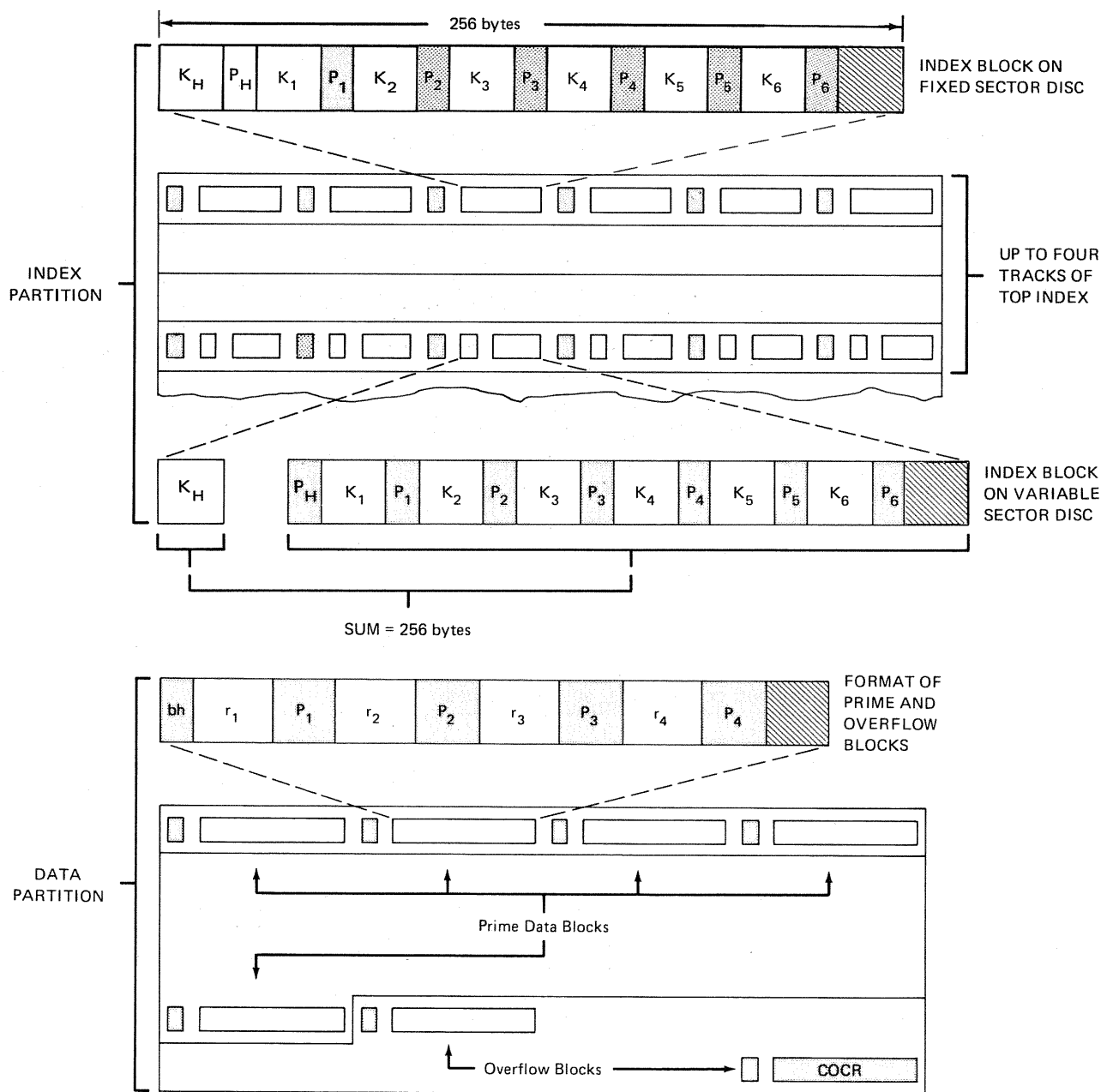
Figure 10—7. OS/3 ISAM File Structure (Part 1 of 2)
